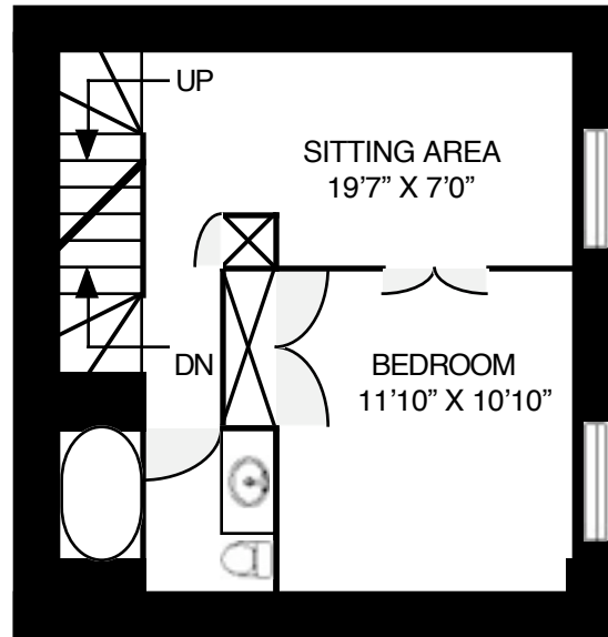
3RD LEVEL - 484 Sq. Ft.
